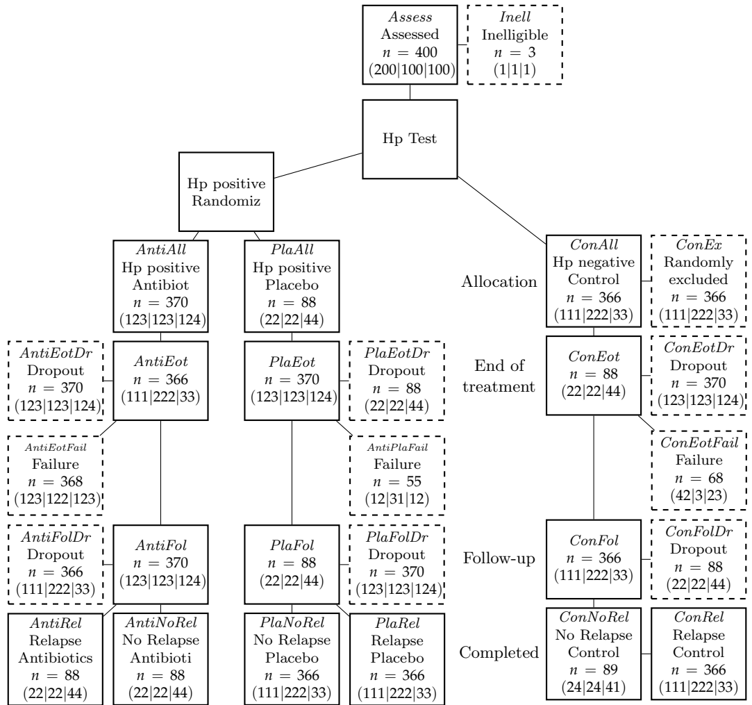
Figure 1: Consort Diagram Example
